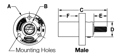
Threaded Stud (Male Shown)
